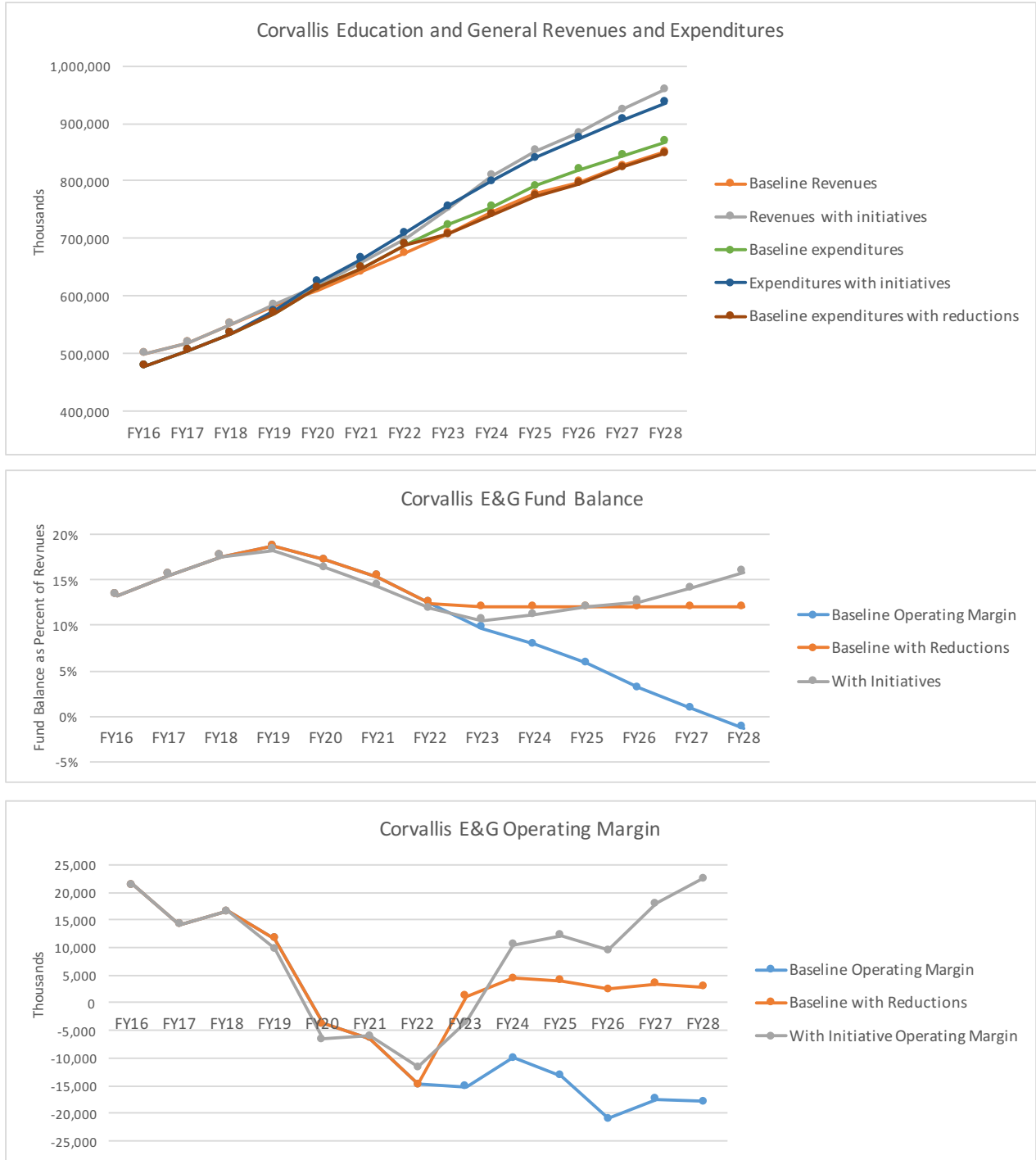
Figure 1: Summary of the ten-year operating forecast for Corvallis Education and General funds. Top is total revenues and expenditures (plus net transfers), middle shows ending fund balances as a percentage of revenues, and bottom shows annual operating balance. The baseline case assumes no additional enrollment initiatives are successful. The baseline with reductions requires sufficient reductions in expenditures to maintain at least a 12% ending fund balance. The “with initiatives” curves assume that the enrollment initiatives in Portland and for an alternate entry to the university are successful.
